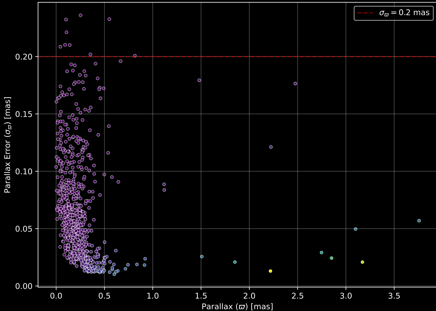
APOGEE DR17 Field: [300+00] Parallax Quality (n= 682)
