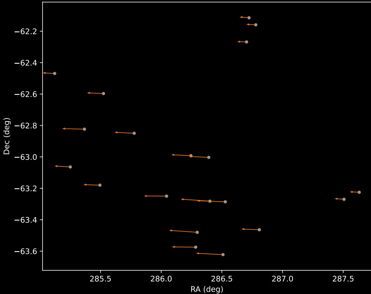
APOGEE DR17 Cluster 22 Proper Motion Vectors (n=20)
