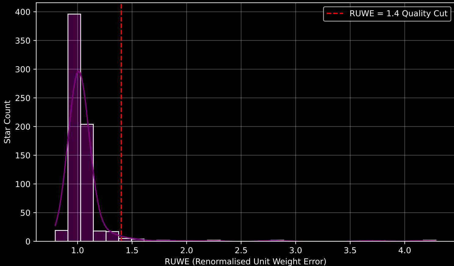
GAPOGEE DR17 Field [300+00] RUWE Distribution (n= 677)
