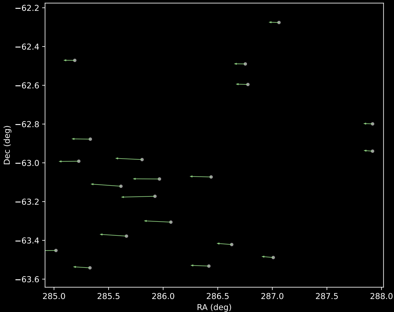
APOGEE DR17 Cluster 25 Proper Motion Vectors (n=20)
