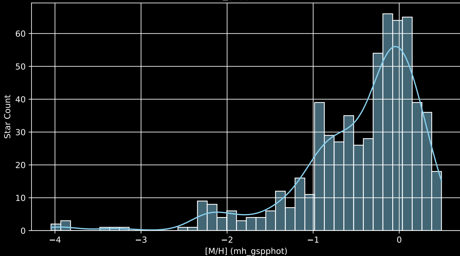
APOGEE DR17 Field: [300+00 [M/H] (mh_gspphot) (n= 626)
