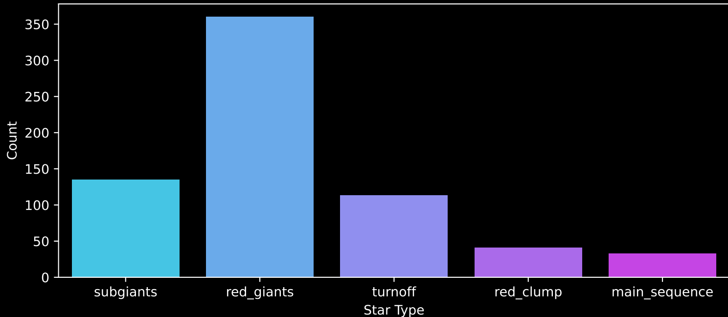
APOGEE DR17 Field: [300+00] Count plot of Star Type
