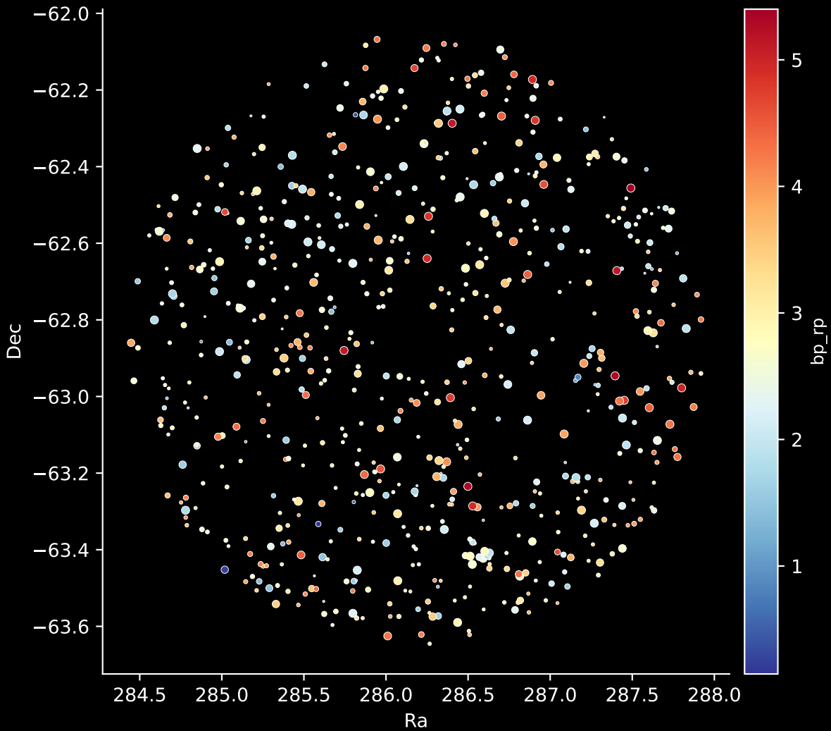
APOGEE DR17 Field: [300+00] Stars: 682
