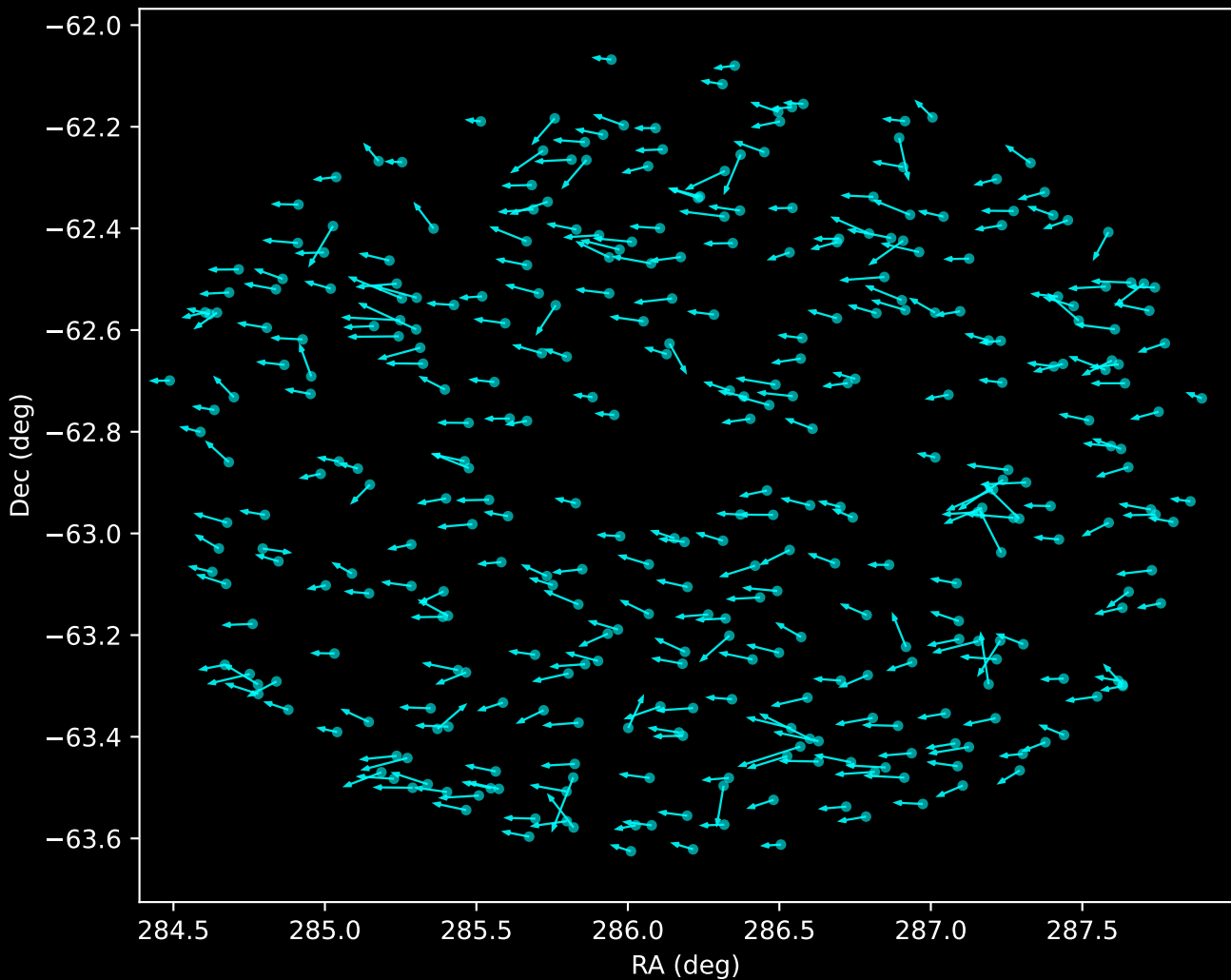
APOGEE DR17 Noise Stream Proper Motion Vectors (n=347)
