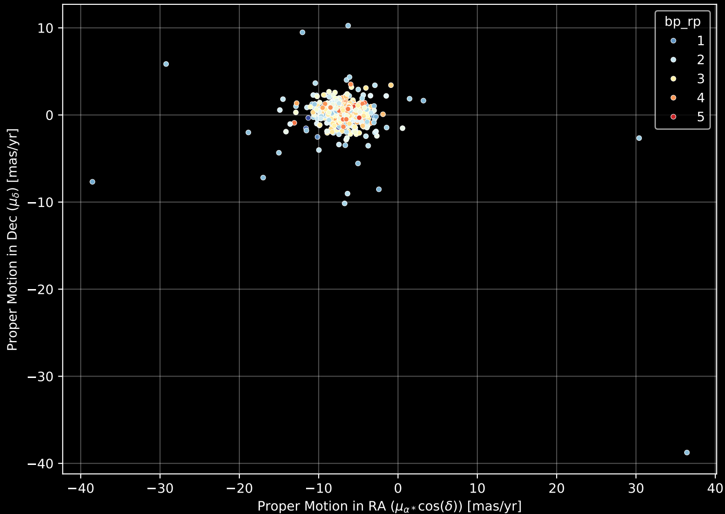
APOGEE DR17 Field: [300+00] Proper Motion Diagram (n= 682)
