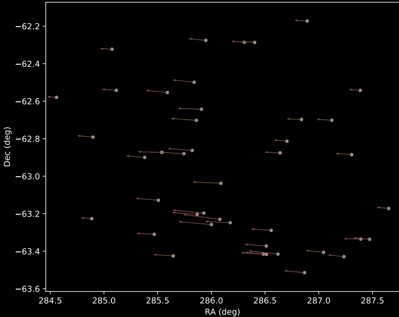
APOGEE DR17 Cluster 30 Proper Motion Vectors (n=43)
